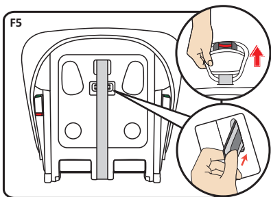
Step 5: Pull out the harness from the slot which under the safety car seat.
