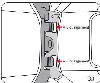
Step 3: Place backrest hooks inside base securely.
